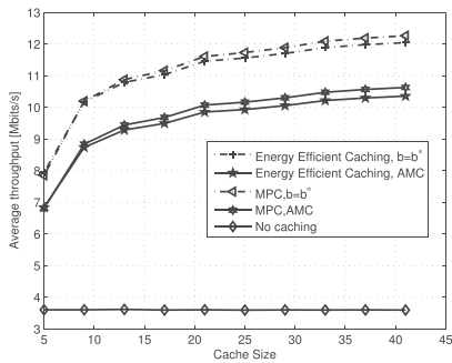
Fig. 6. Average throughput versus the cache size, for M = 5 and N_m = 12 .
