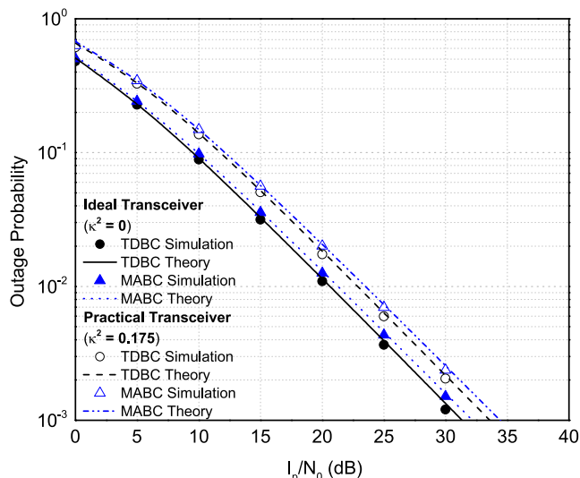
FIGURE 8. OP at A (or at B) of DS-TSB network with respect to I_p/N_0 .
