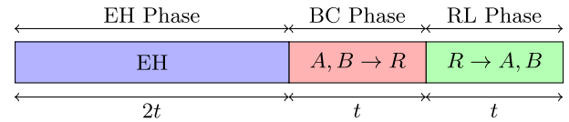
FIGURE 5. Data frame structure of the DS-MABC-TSB network.
