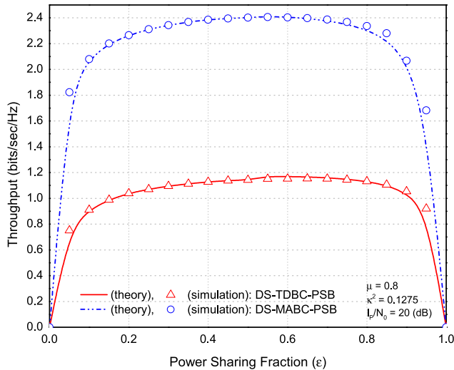
FIGURE 16. Throughput with respect to \epsilon for the PSB receiver architecture.
