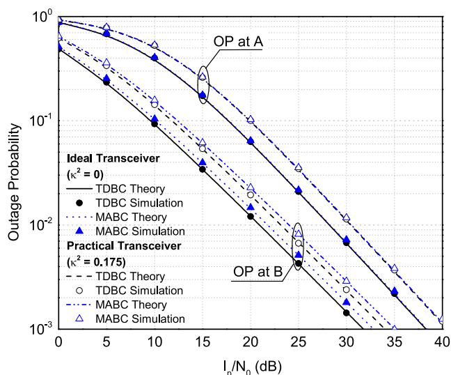
FIGURE 9. OP at A of SFS-TSB network with respect to I_p/N_0 .
