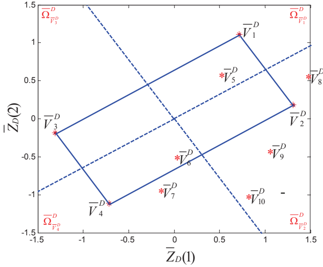
Fig. 4. Received constellation at destination after coordinate transformation.
