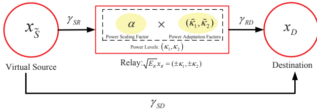
Fig. 5. Virtual channel model. In particular, the channel gains \gamma_{SR} and \gamma_{SD} with respect to virtual channels will be introduced in detail in the following paragraph. x_{\bar{S}} is the virtual source message, which is generated from the original transmitted signal as x_{\bar{S}} = x_1 \boxplus x_2 . x_{\mathcal{R}} is the real transmitted signal from the relay to destination. And x_{\mathcal{D}} is also equal to x_1 \boxplus x_2 .
